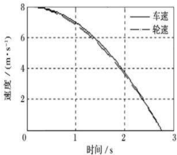
(a) no anti-skid braking control
