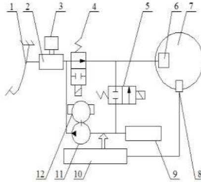
Figure 2: Anti Lock Braking System Schematic
