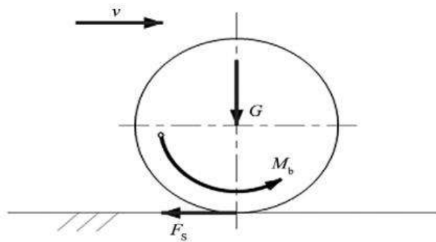
Figure 4: Single Wheel Force
