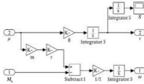
Figure 5: Vehicle Dynamics Model
