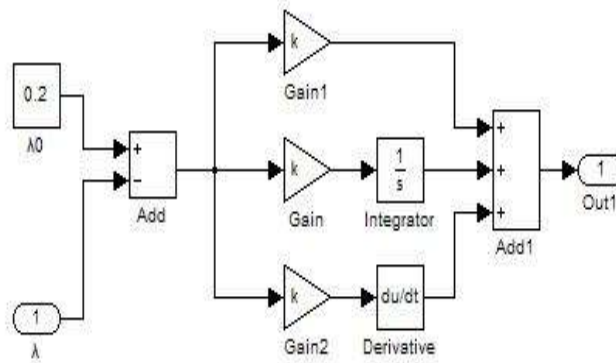
Figure 8: PID Control Module
