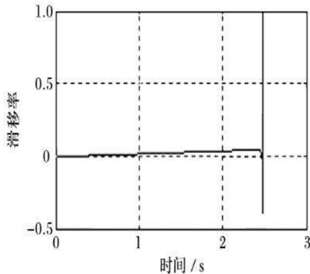
(b) logical threshold control
