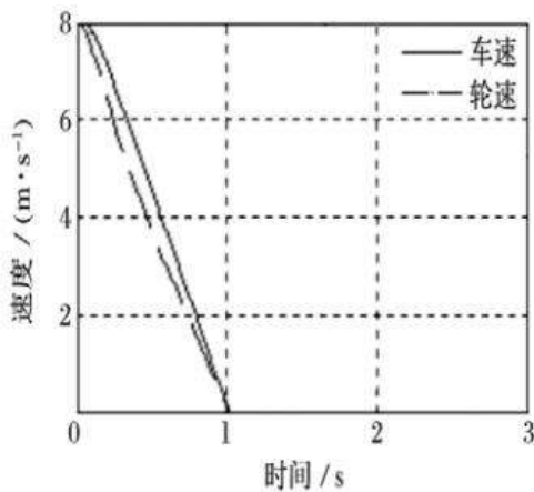
(c) PID control
