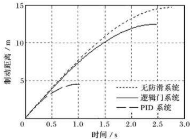
Figure 9: Braking Distance of Electric Locomotive
