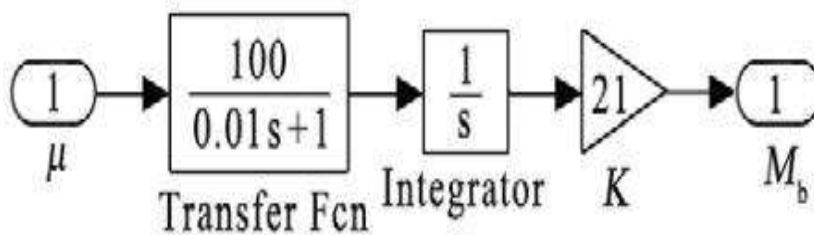
Figure 6: Brake System Model
