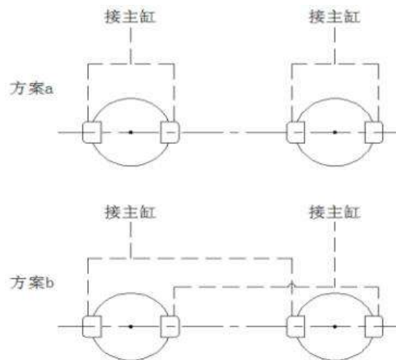
Figure 3: Braking Shunt Scheme
