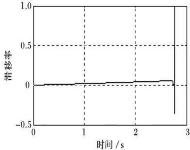
(a) no anti-skid braking control
